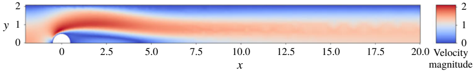
FIGURE 7. (Colour online) Illustration of the converged flow obtained around a centred half-domain, using a symmetric boundary condition at the lower boundary. The lower boundary cuts the cylinder through its equatorial plane. This results in a configuration where no vortex shedding is present, which constitutes a ‘hypothetical’ no-shedding baseline to which we can compare our results. The mesh is heavily refined in all the recirculation area.
